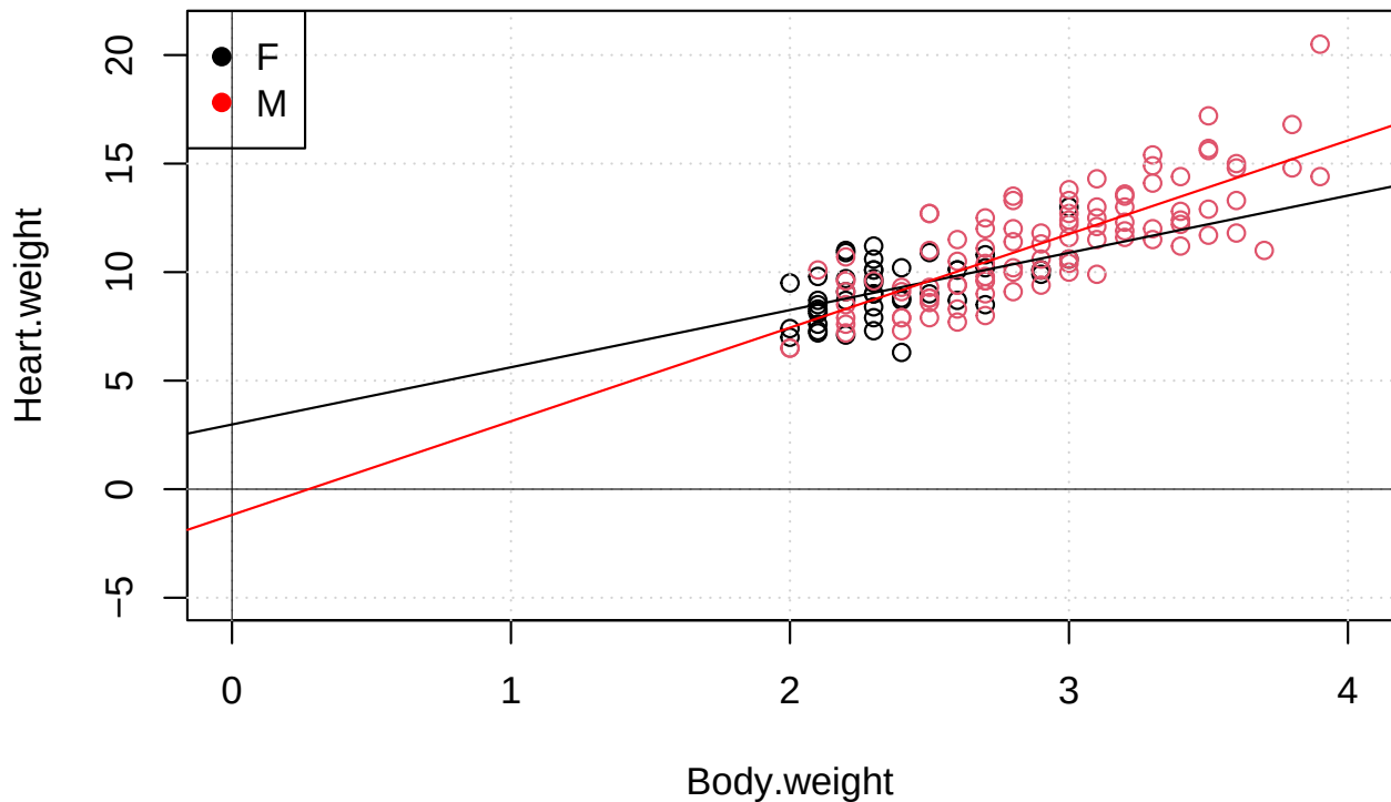
Model 'lm.cats.3'
